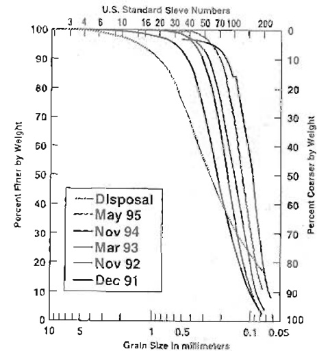
Figure 4. Grain Size Distribution Comparison, Line 19, d = -24 ft
